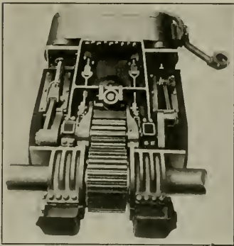
TWO-CYLINDER ENGINE GEARED TO THE TRAILER AXLE
